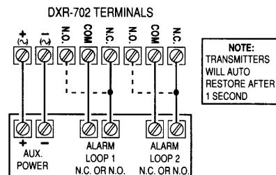
ALARM PANEL CONNECTION FOR PANIC BUTTONS 1 SECOND RELAY OPTION
